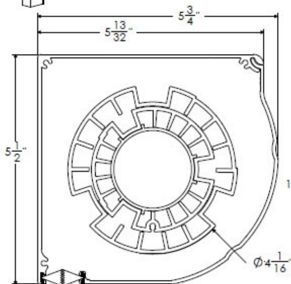
SRS Series 5 Housing
