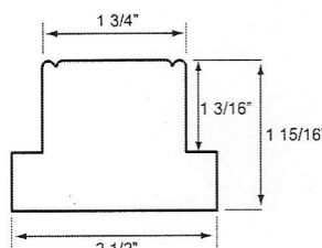
LARGE T-POST
