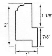
ATLANTA Z-FRAME
