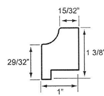
HOWE CASE
