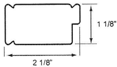
RABBETED STILE
