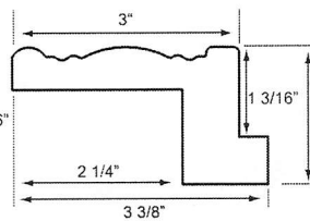
LARGE Z-FRAME
