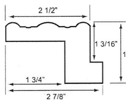
MEDIUM Z-FRAME
