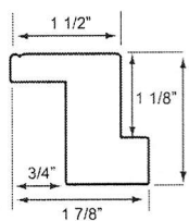
SINGLE BEADED Z-FRAME
