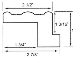
MEDIUM Z-FRAME
