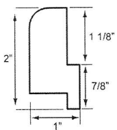
CHICAGO Z-FRAME
