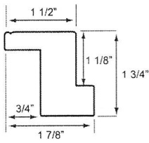
SINGLE BEADED Z-FRAME
