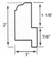
ATLANTA Z-FRAME
